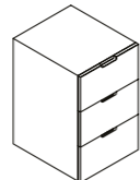
DU Drawer unit W400 D250/525 H700 mm
